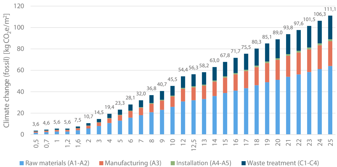
Figure 3 Climate change (fossil) impact across Lamitech Laminate thicknesses
