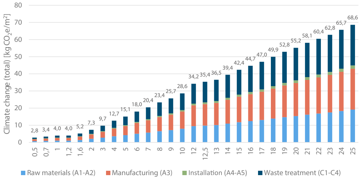
Figure 2 Climate change (total) impact across Lamitech Laminate thicknesses
